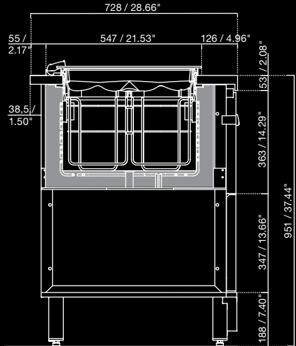
Banco PANORAMA senza riserva PANORAMA counter with one level of gelato tubs Comptoir PANORAMA sans réserve PANORAMA-Theke ohne Vorrat Mostrador PANORAMA sin reserva
